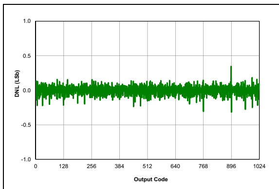
FIGURE 38-45: ADC, DNL, V_{DD} = 3.0V , T_{AD} = 1\text{ }\mu\text{S} , 25^\circ\text{C} .
