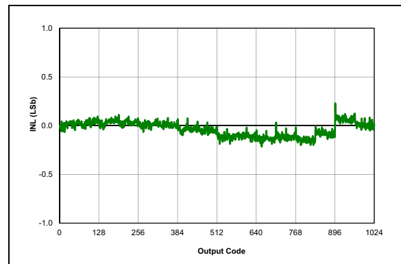
FIGURE 38-48: ADC, INL, V_{DD} = 3.0V , T_{AD} = 4\text{ }\mu\text{S} , 25^\circ\text{C} .
