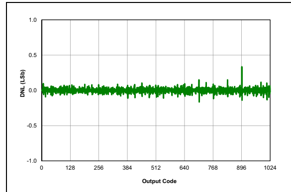
FIGURE 38-46: ADC, DNL, V_{DD} = 3.0V , T_{AD} = 4\text{ }\mu\text{S} , 25^\circ\text{C} .
