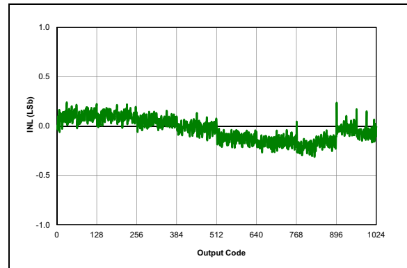
FIGURE 38-47: ADC, INL, V_{DD} = 3.0V , T_{AD} = 1\text{ }\mu\text{S} , 25^\circ\text{C} .
